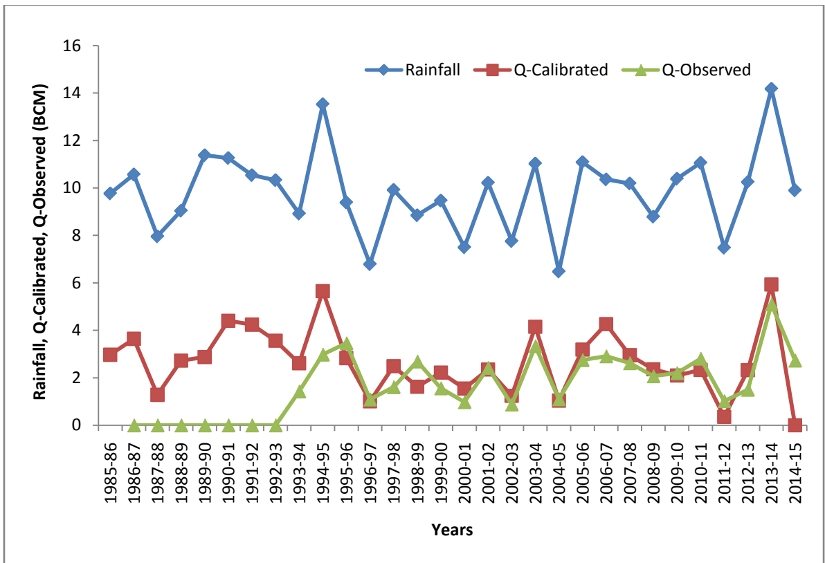
Figure 8.17 Calibrated runoff and observed discharge at Purushottampur
