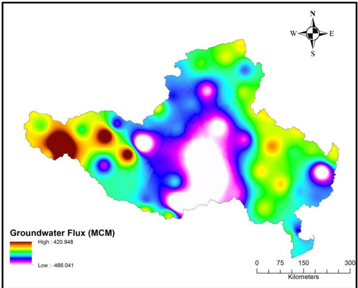
Figure 1.10 Groundwater flux (spatial data) estimated during 2002-03
