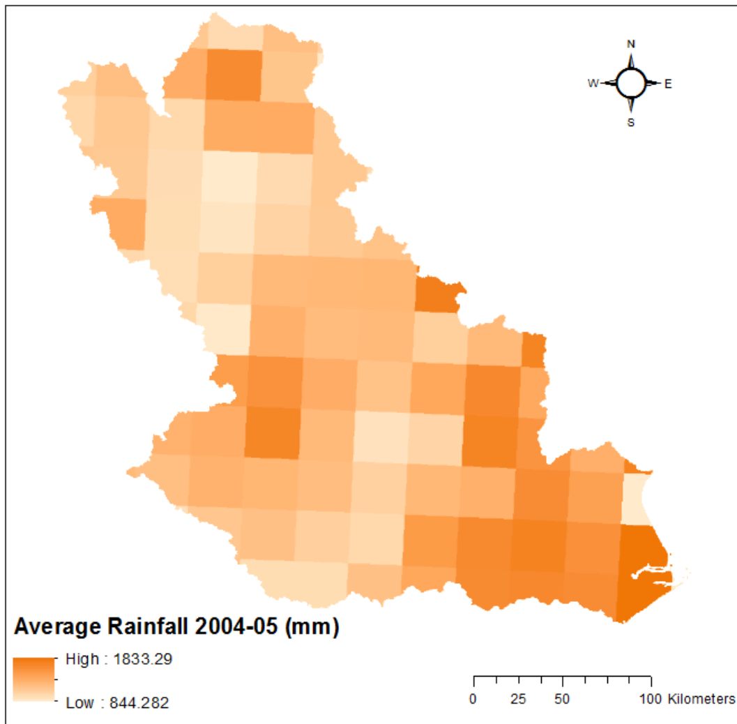
Figure 5.5 Gridded rainfall of Brahmani-Baitarani basin (2004-05)
