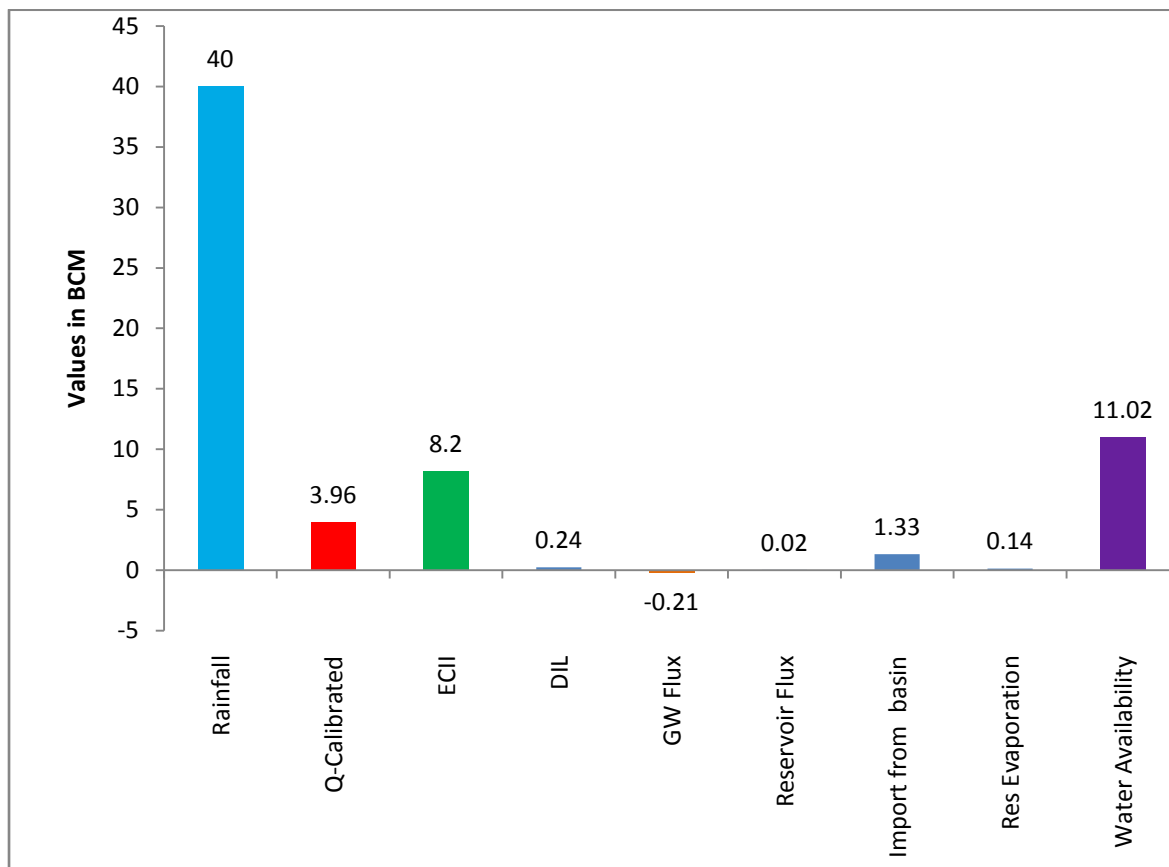
Figure 7.18 Mean water balance components of Pennar basin
