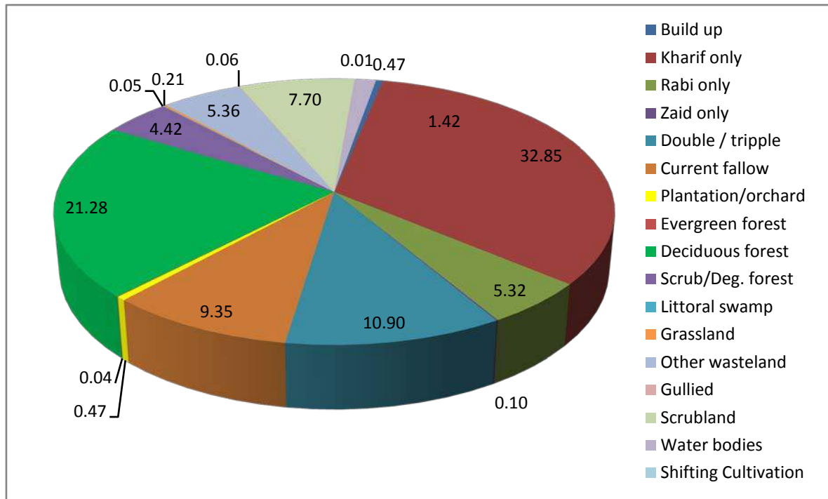
Figure 1.2 Distribution of LULC in Godavari basin (2004-05)
