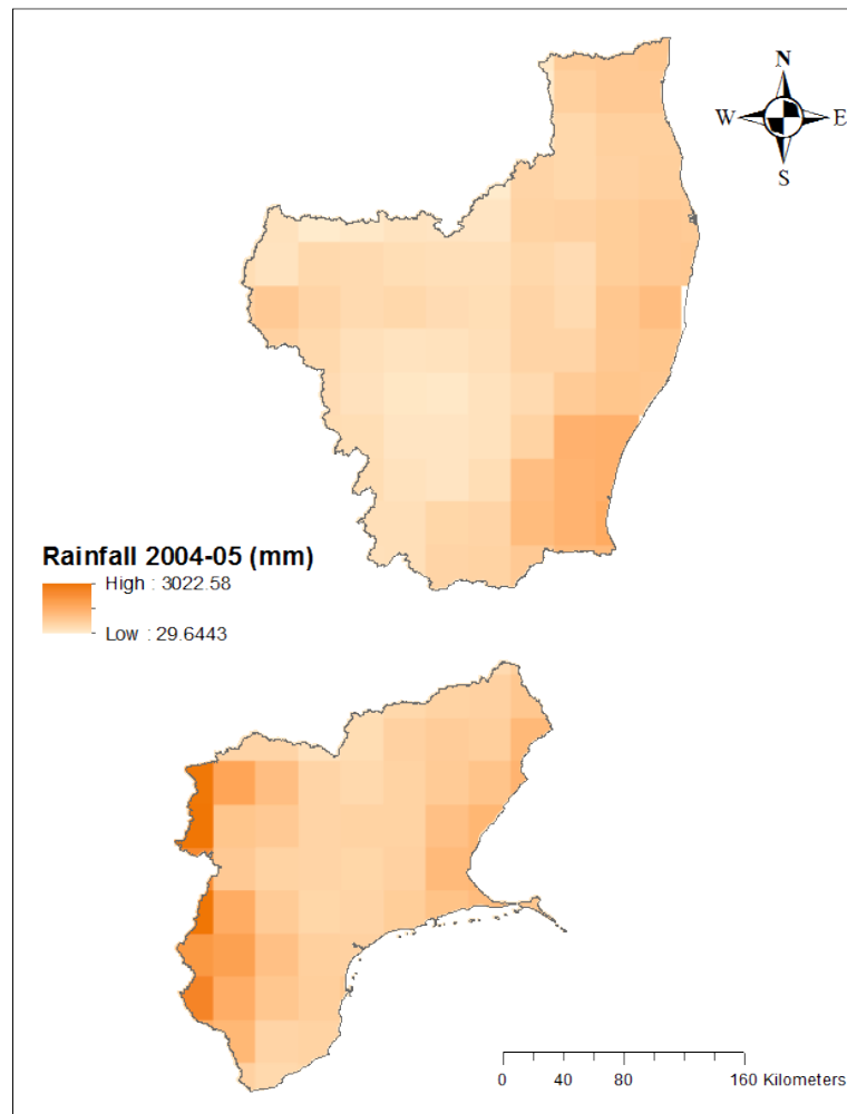
Figure 9.5 Gridded rainfall of EFR between Pennar and Kanyakumari basin (2004-05)
