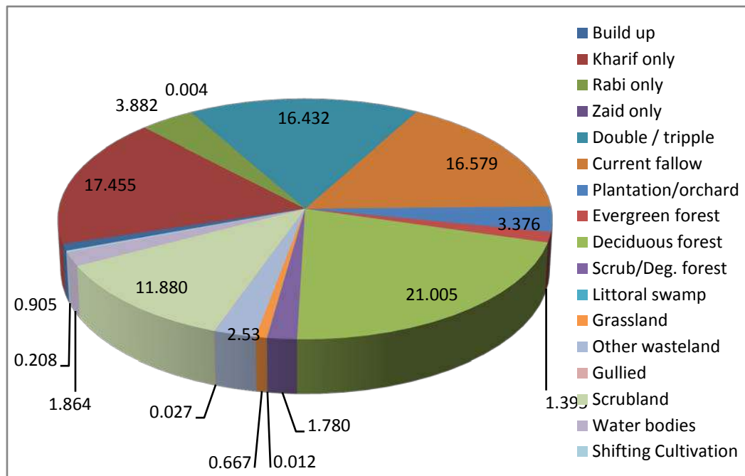
Figure 8.2 Distribution of LULC in EFR between Mahanadi and Pennar basin (2004-05)
