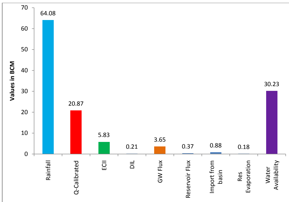
Figure 7.16 Water balance components of Pennar basin during extreme high rainfall (1996-97)
