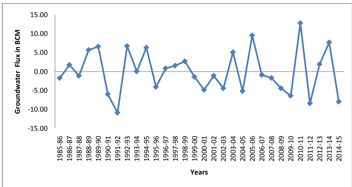
Figure 1.11 Annual groundwater flux of Godavari basin (1985-86 to 2014-15)
