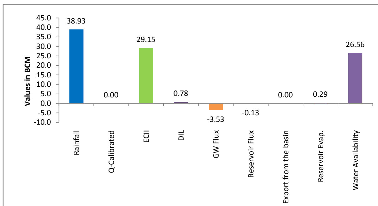
Figure 3.17 Water balance components of Cauvery basin during extreme low rainfall (2002-03)
