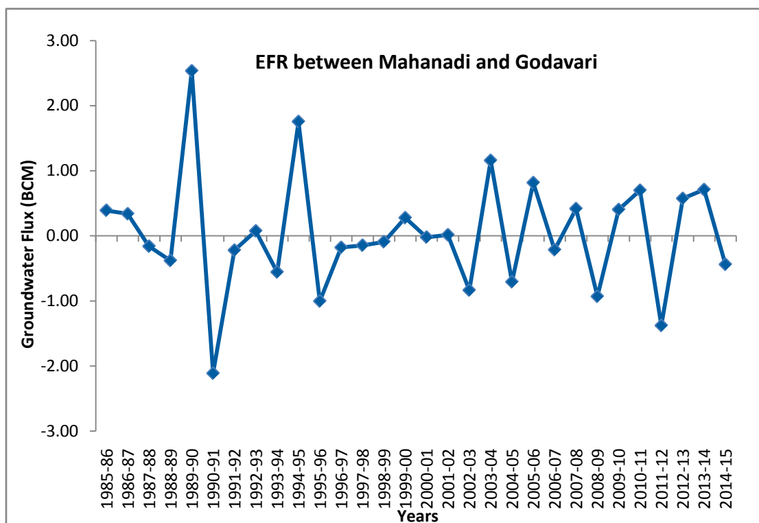
Figure 8.11(a) Annual groundwater flux of EFR between Mahanadi and Godavari basin (1985-1986 to 2014-15)
