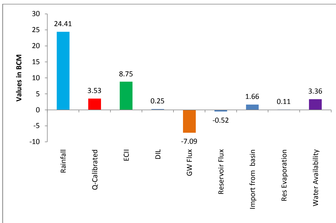
Figure 7.17 Water balance components of Pennar basin during extreme low rainfall (2002-03)
