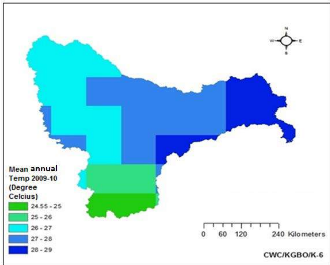
Figure 2.7 Gridded mean annual temperature of Krishna basin (2009-10)
