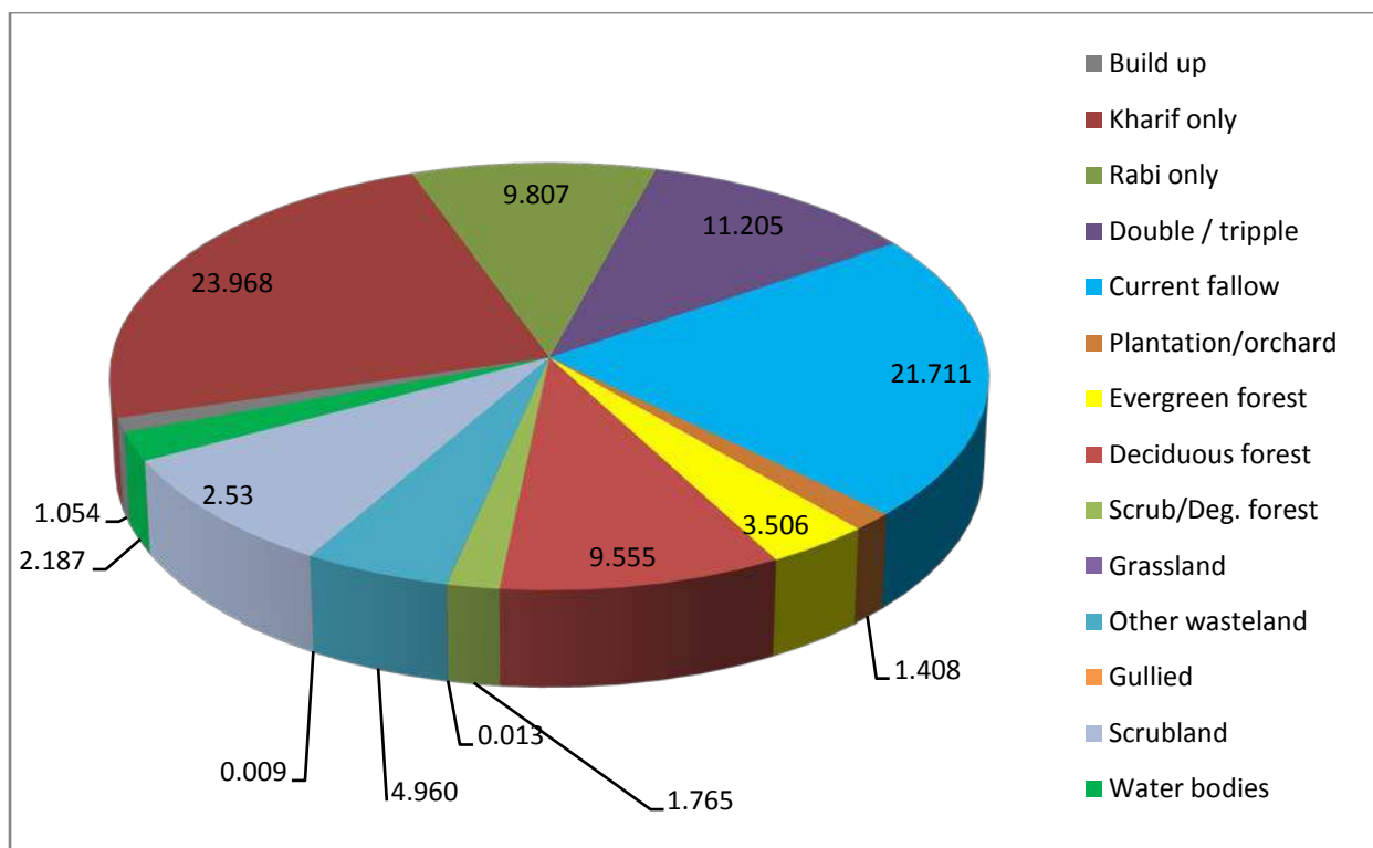
Figure 9.2 Distribution of LULC in EFR between Pennar and Kanyakumari basin (2004-05)
