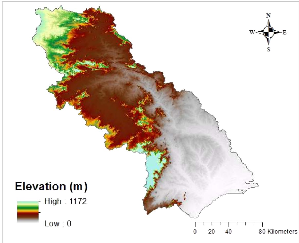
Figure 4.4 SRTM DEM map of Subernarekha basin
