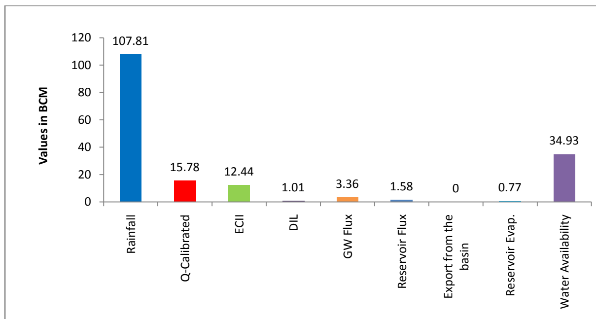
Figure 3.16 Water balance components of Cauvery basin during extreme high rainfall (2010-11)
