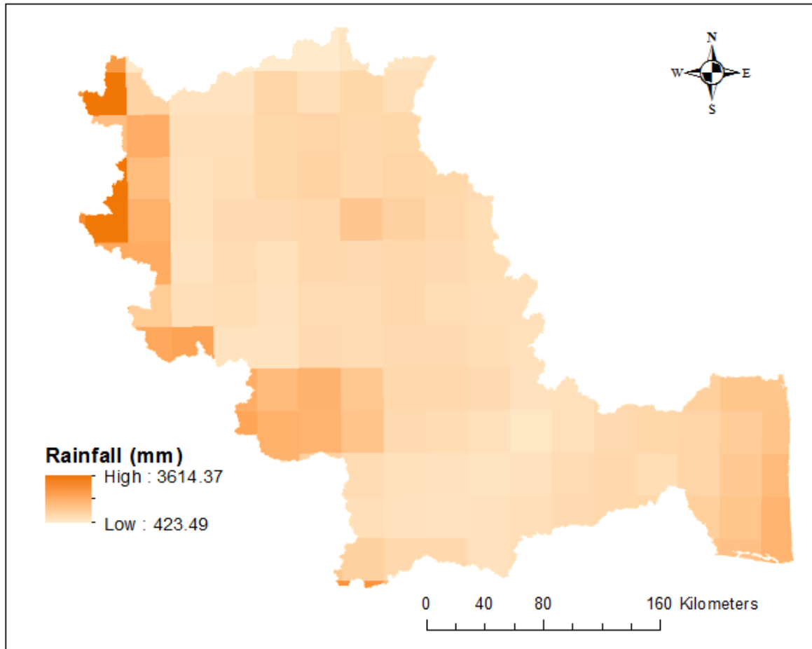
Figure 3.5 Gridded rainfall of Cauvery basin (2004-05)
