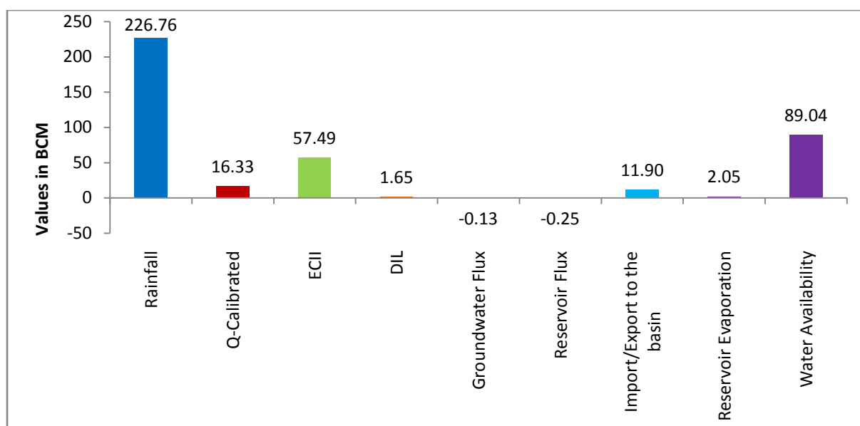
Figure 2.23 Mean water balance components of Krishna basin (mean of 29 years)
