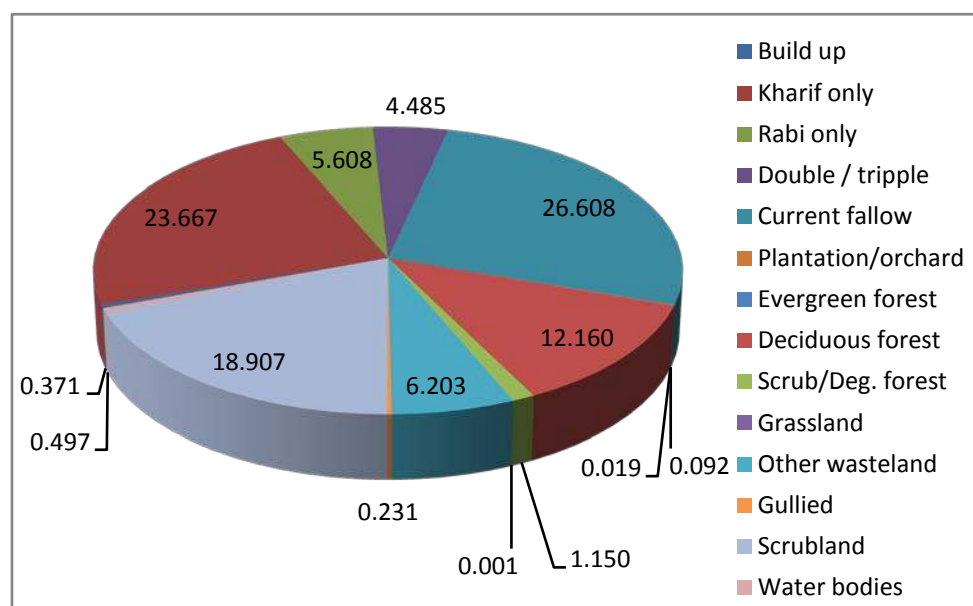
Figure 7.2 Distribution of LULC in Pennar basin (2004-05)
