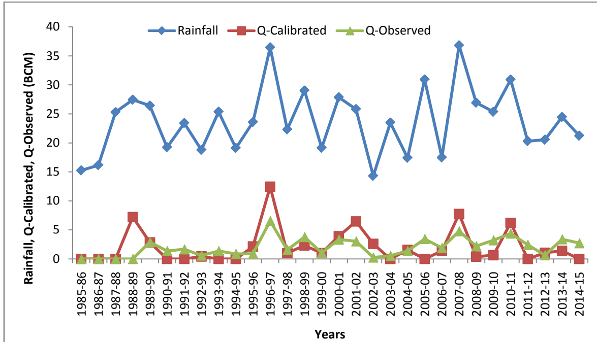
Figure 7.14 Calibrated runoff and observed discharge at Chennur
