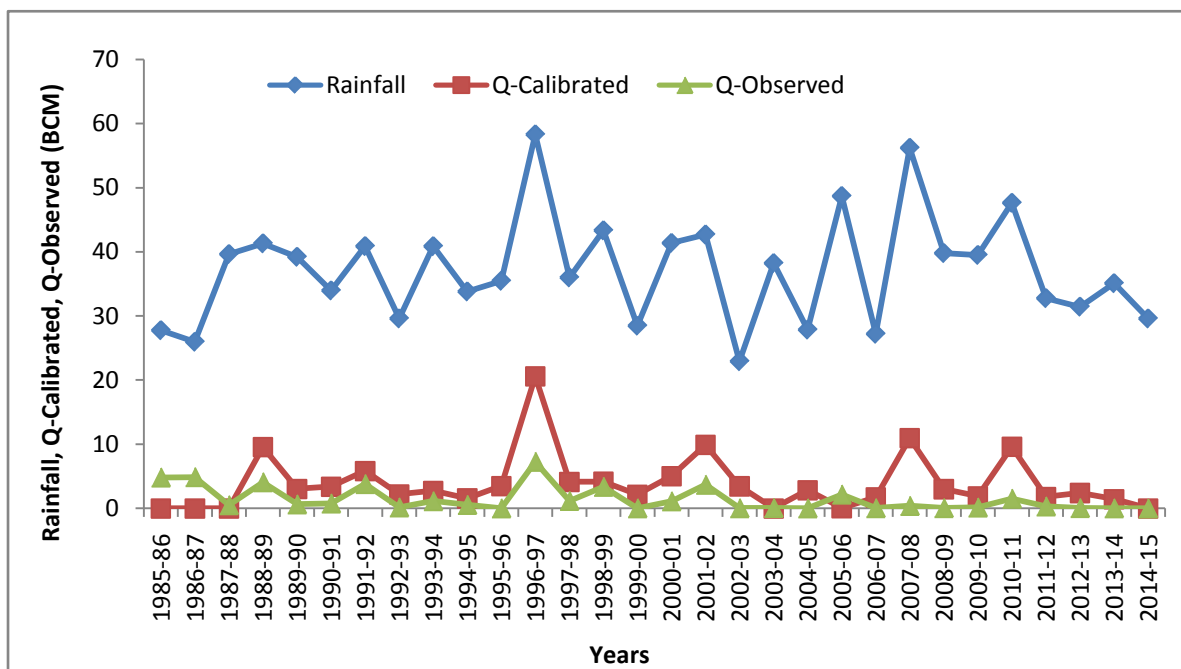
Figure 7.15 Calibrated runoff and observed discharge at Nellore
