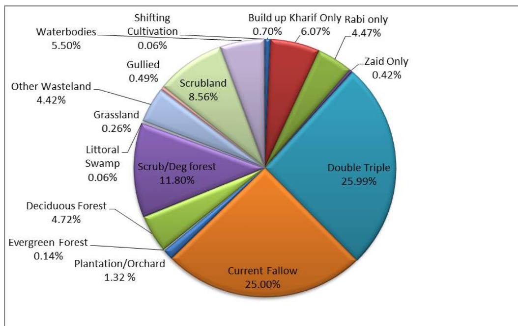
Figure 6.2 Distribution of LULC in Mahanadi basin (2004-05)
