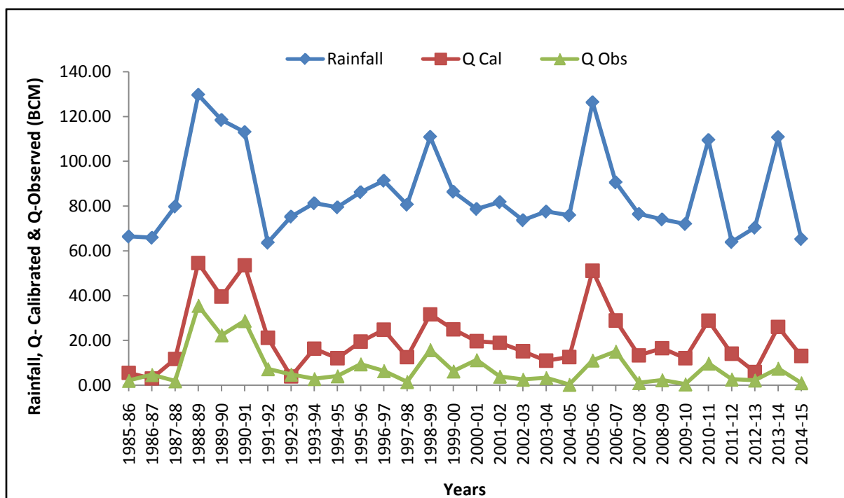
Figure 1.17 Calibrated runoff and observed discharge at Mancharial
