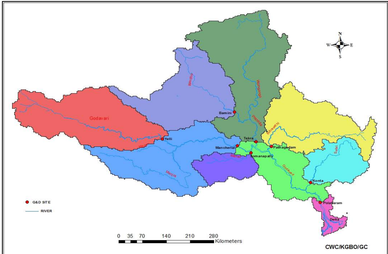
Figure 1.8 Sub-basins of Godavari basin
