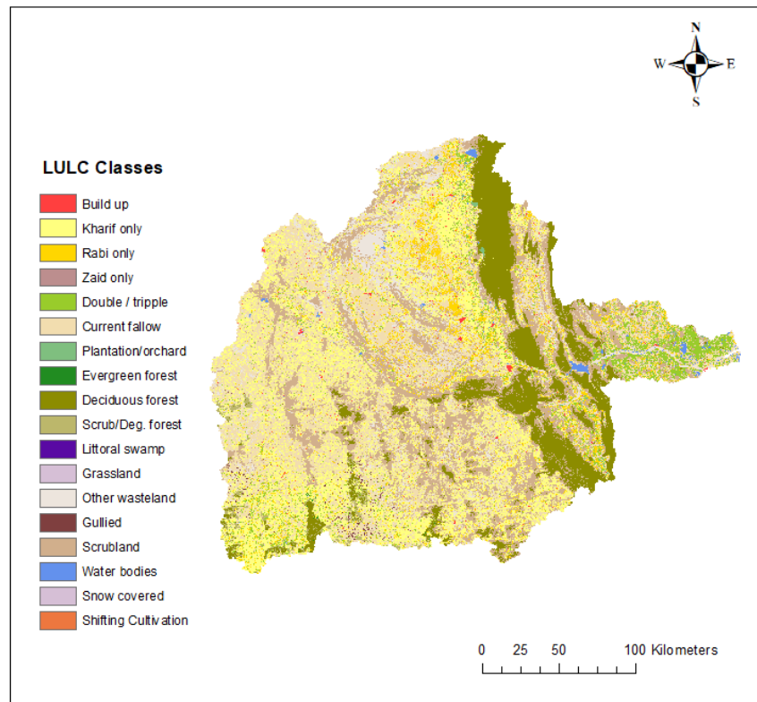
Figure 7.1 LULC Map of Pennar basin (2004-05)
