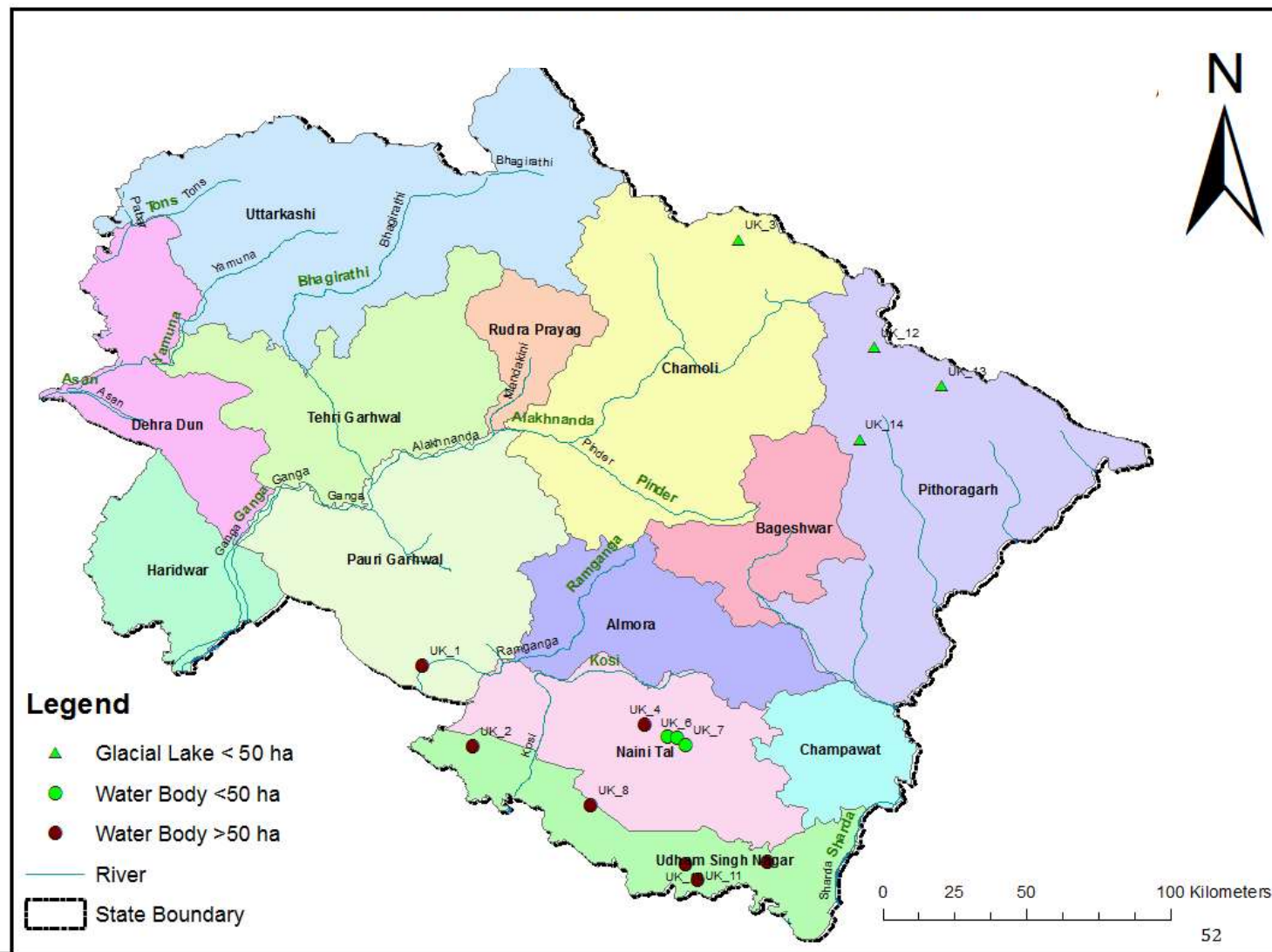
Figure 3 (d): Glacial Lakes & Water Bodies in Uttarakhand
