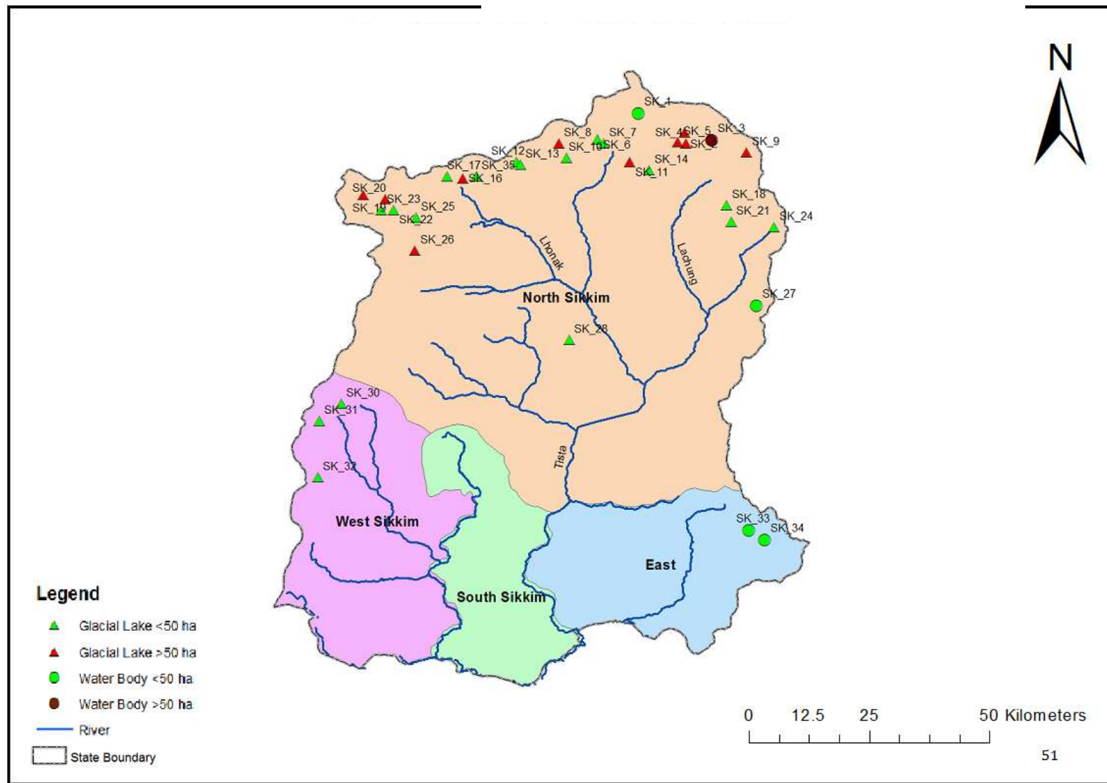
Figure 3 (c): Glacial Lakes & Water Bodies in Sikkim
