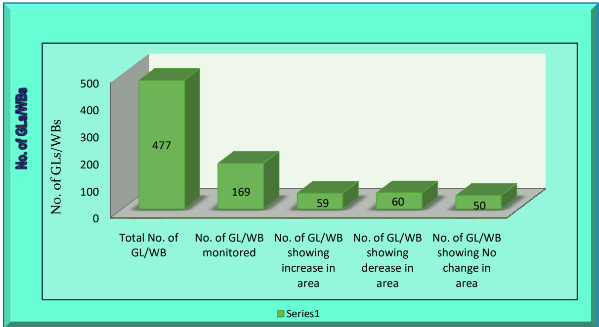
Figure 2: Glacial Lakes/ Water Bodies Monitored during the month July 2021
