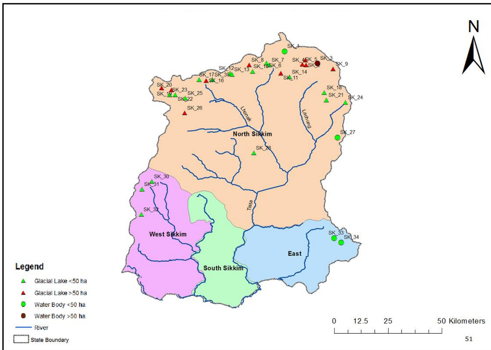
Figure 3 (c): Glacial Lakes & Water Bodies in Sikkim
