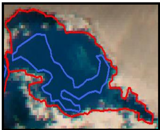
Figure 3 (f): Satellite Imageries of GL & WB that have shown INCREASE in water spread area ( > 40\% )
