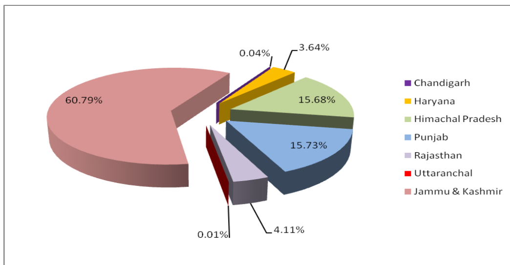
Figure 3.14 Percentage area of Indus basin in various States
