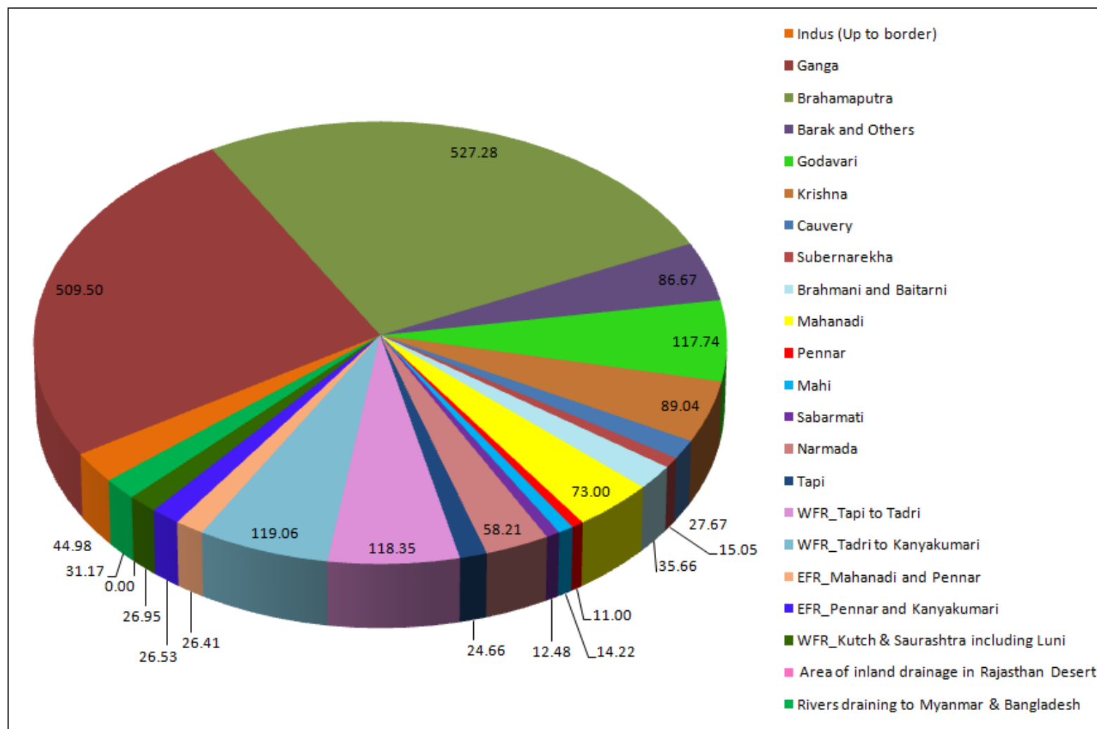
Figure 4.1 Water availability in various river basins of India
