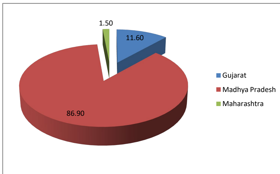
Figure 3.27 Percentage area of Narmada basin in various States
