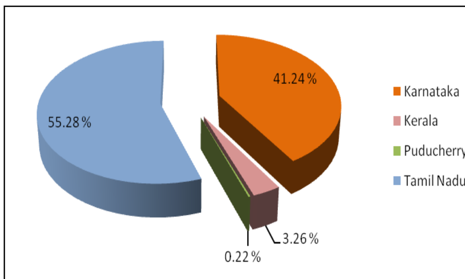
Figure 3.20 Percentage area of Cauvery basin in various States
