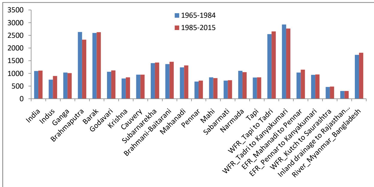
Figure 4.4 Comparison of Rainfall between (1965-1984) and (1985-2015)
