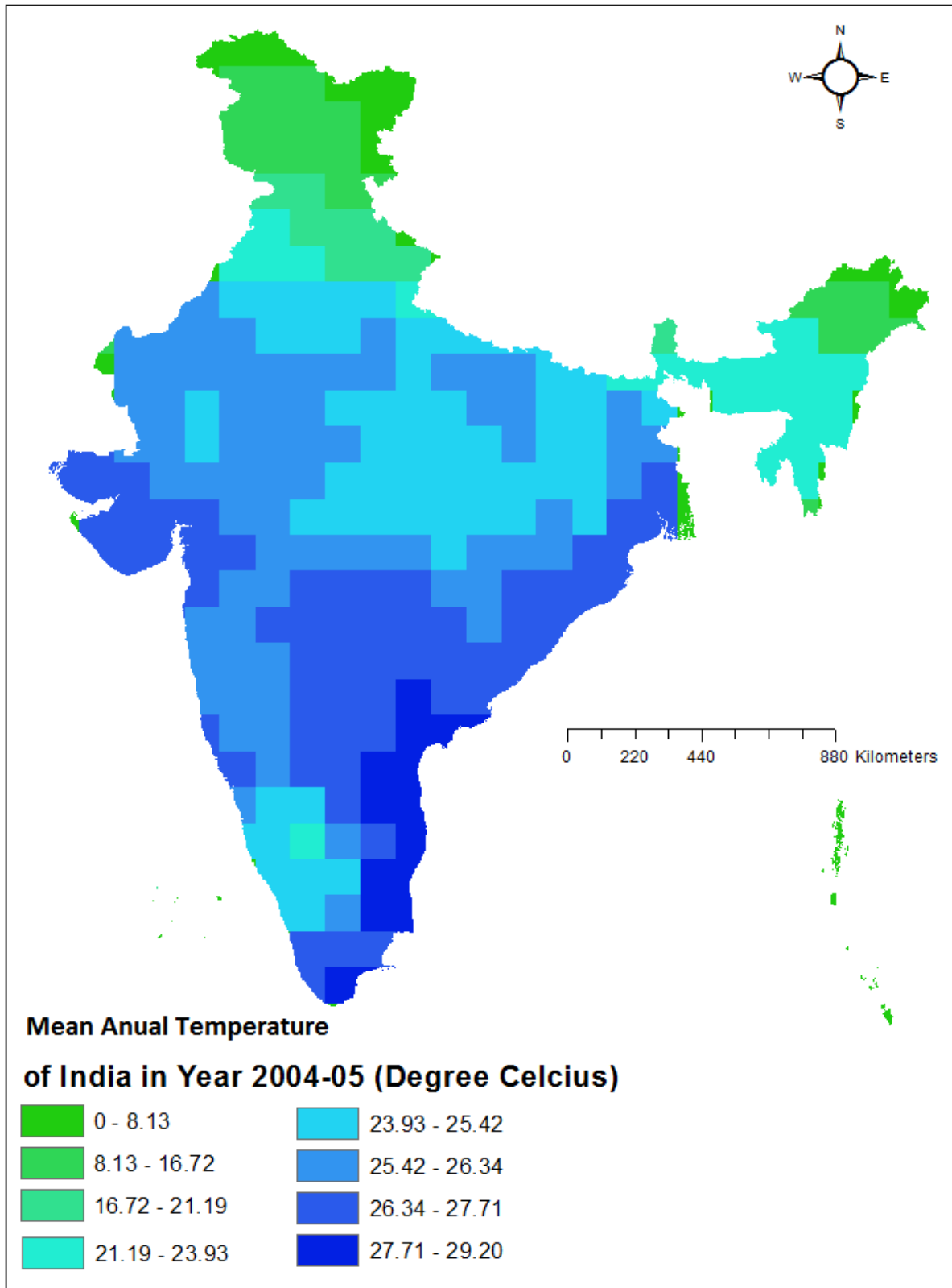
Figure 3.7 Gridded mean annual temperature of India (2004-05)
