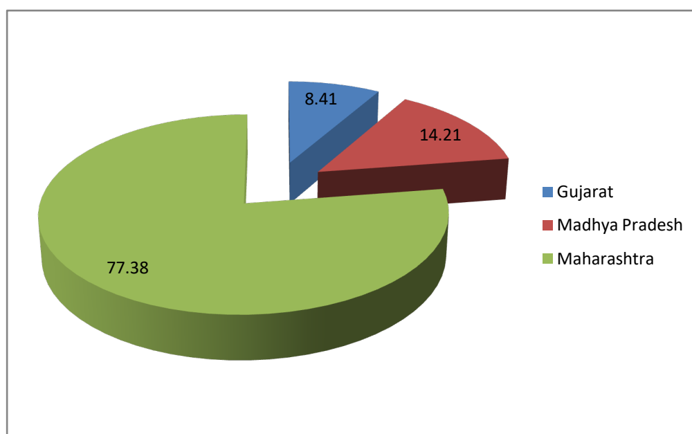
Figure 3.28 Percentage area of Tapi basin in various States
