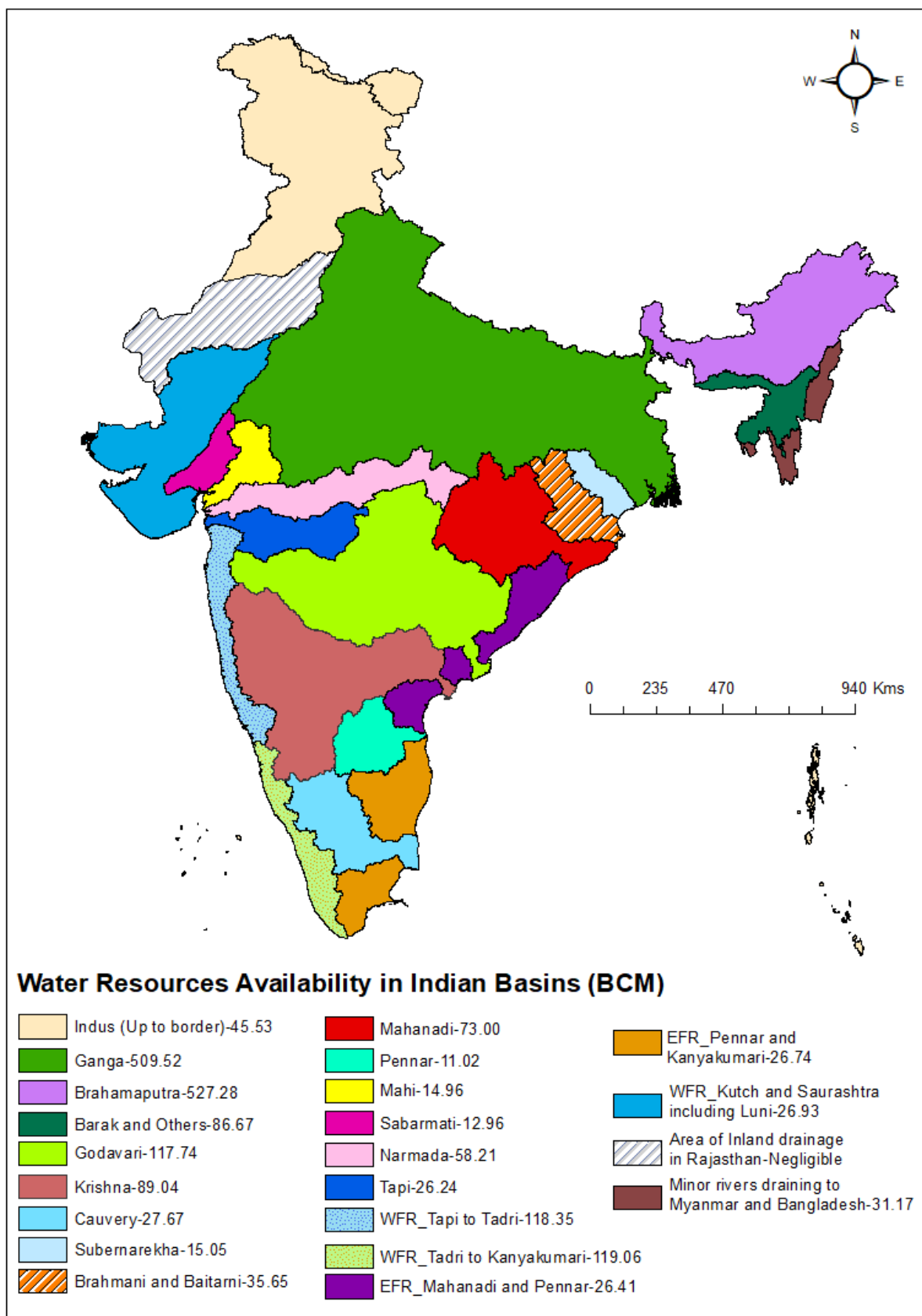
Figure 4.2 Map of basin-wise water availability in India
