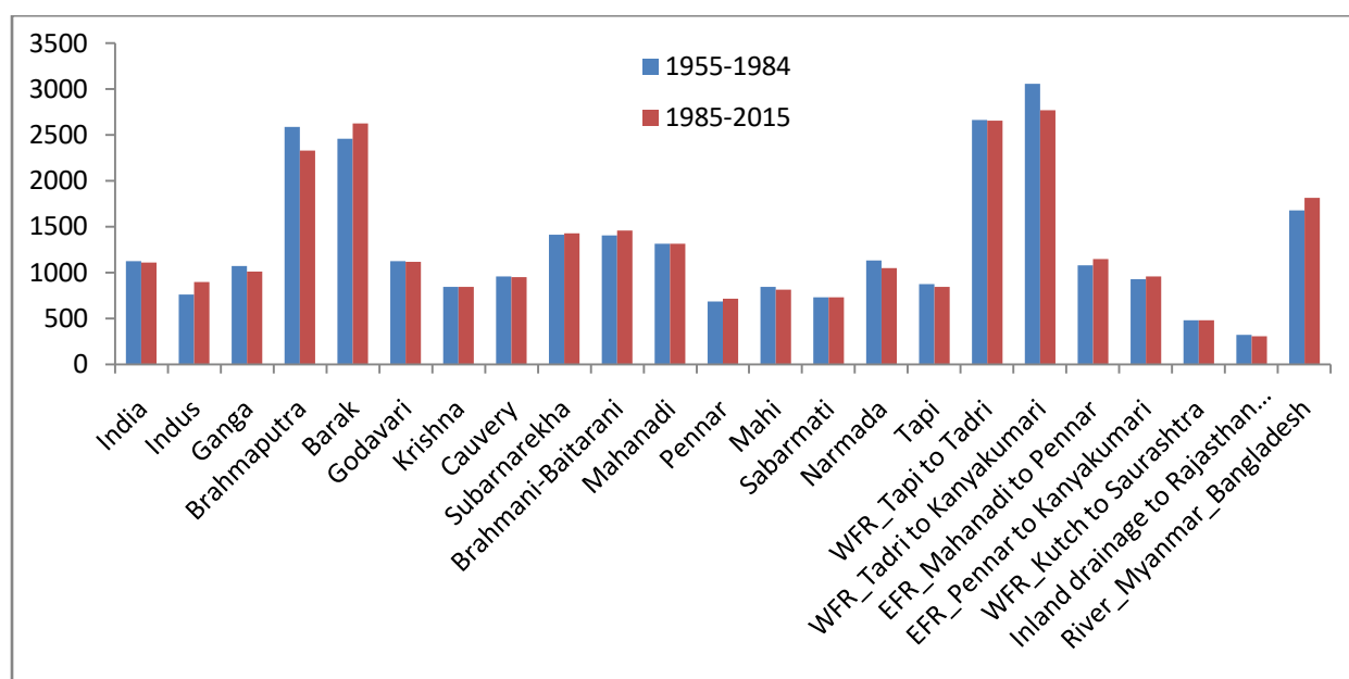
Figure 4.3 Comparison of Rainfall between (1955-1984) and (1985-2015)
