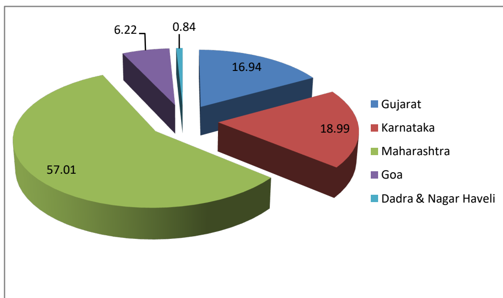
Figure 3.29 Percentage area of WFR from Tapi to Tadri basin in various States
